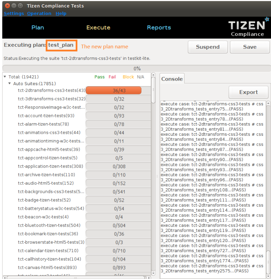
Figure 3-5: Execute a New Auto Test Plan
