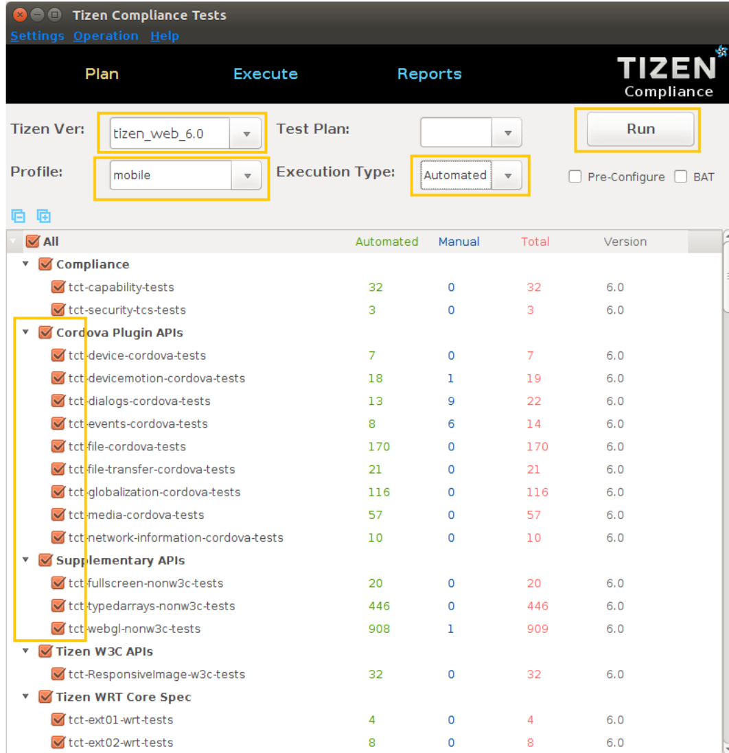
Figure 3-2a: Change Auto Test Plan
