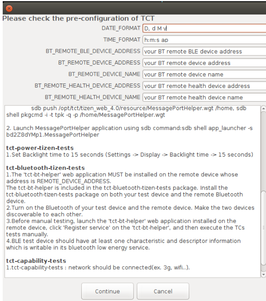
Figure 3-7: Web TCT Manager Pre-configuration Page
