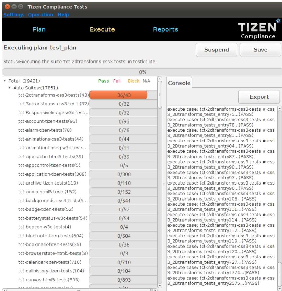
Figure 3-8: Web TCT Manager Execution UI Page
