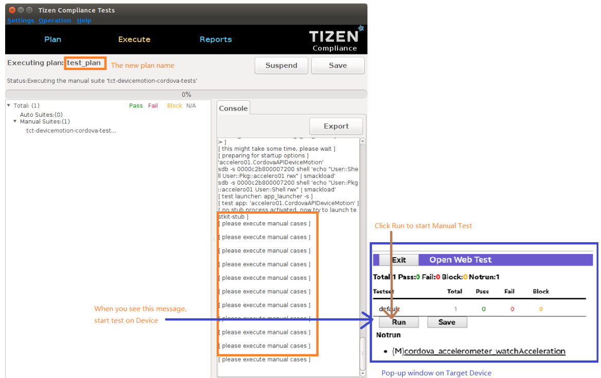
Figure 3-6a: Execute a New Manual Test Plan
